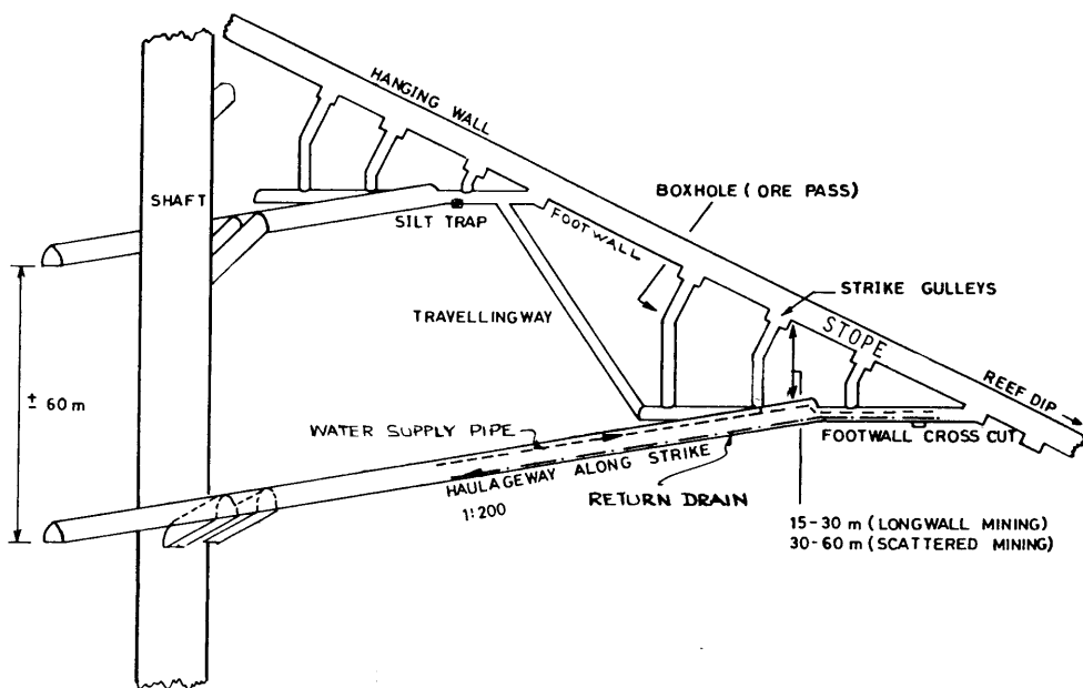
DIAGRAMATIC ELEVATION OF WORKINGS.
