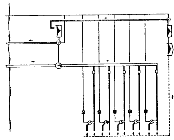
B. Turbines & head control valves
